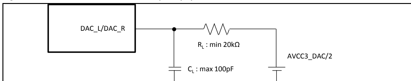
Figure 8-9: R_L is Connected to AVCC3_DAC/2 (Example)
