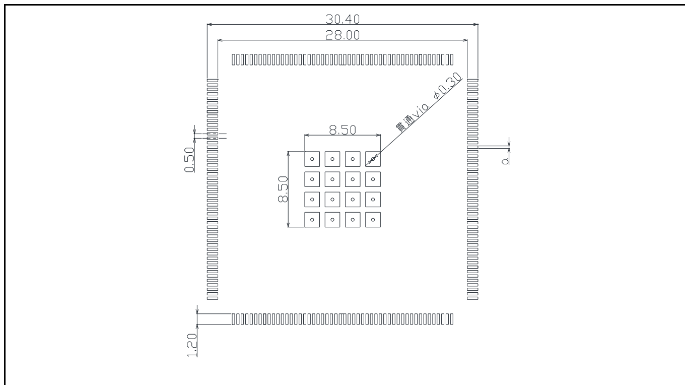
Figure 8-3: Land Pattern and Thermal Via LET208
