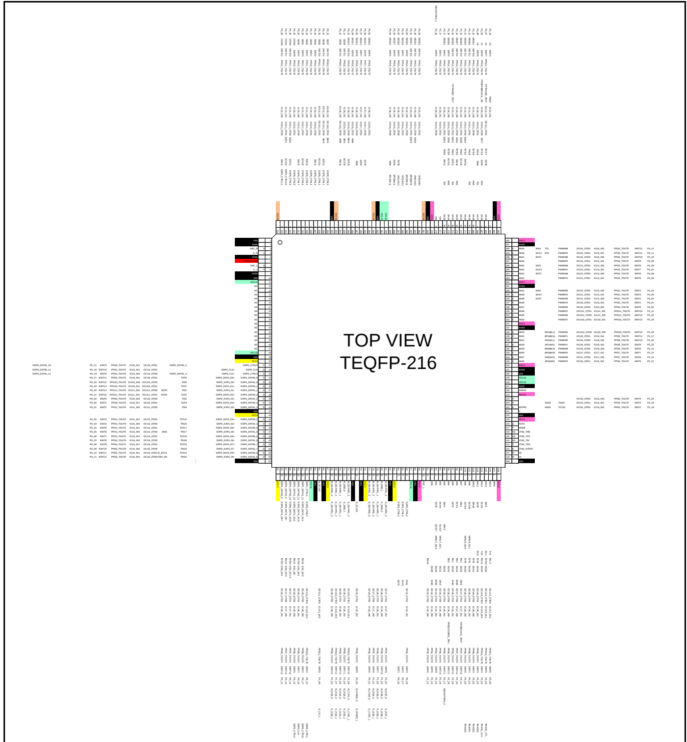
Figure 4-8: TEQFP-216
