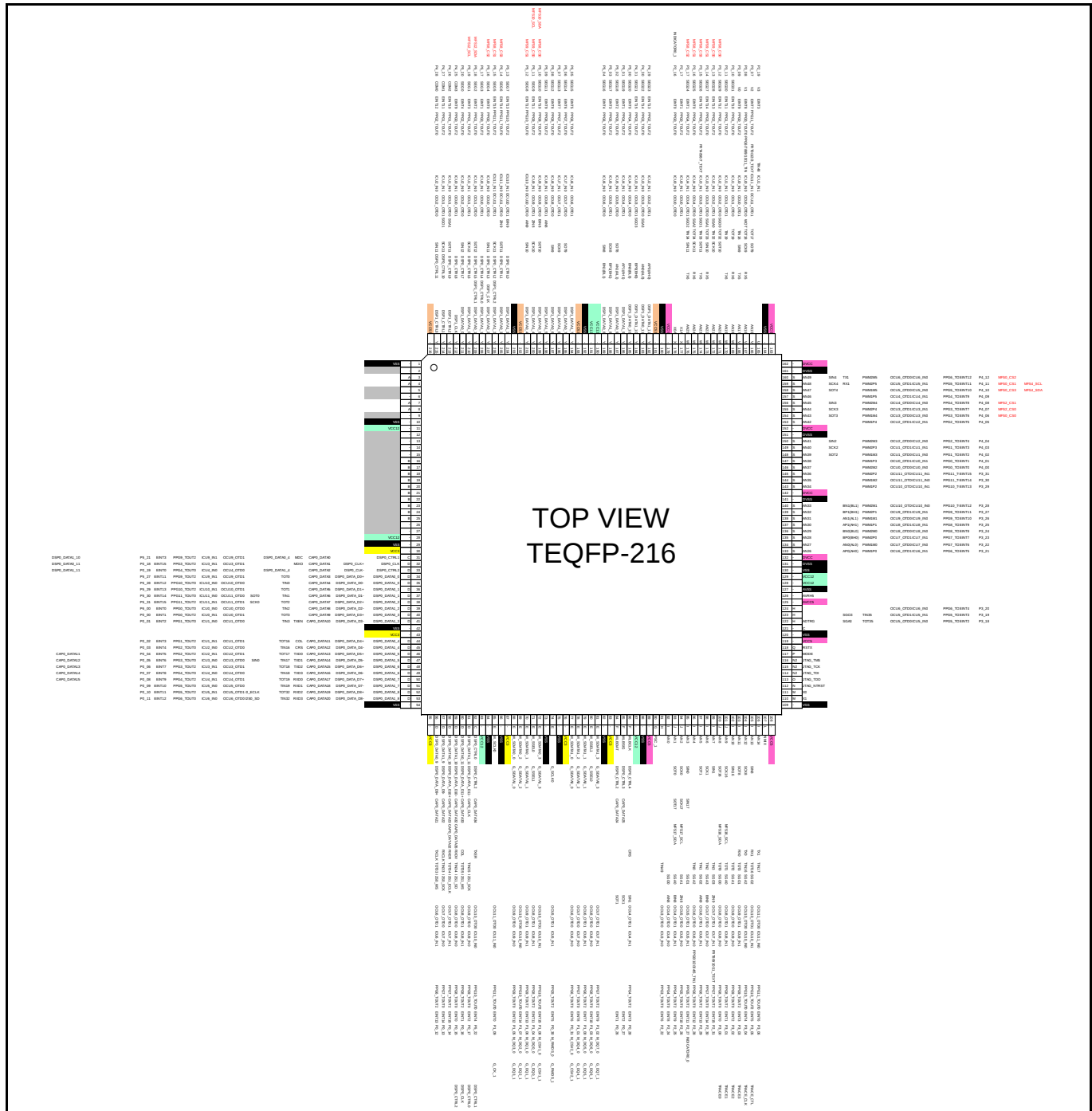
Figure 4-7: TEQFP-216 (S6J323CLxx)
