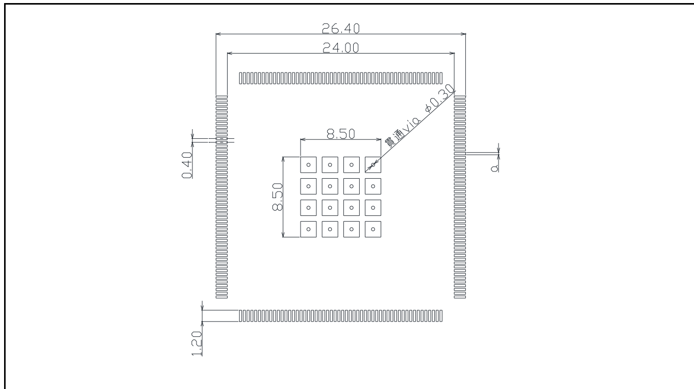
Figure 8-2: Land Pattern and Thermal Via LEQ216
